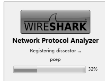
图3-2 WireShark
