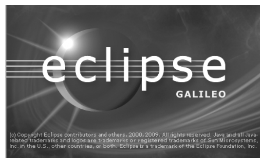
图3-1 Eclipse Galileo
